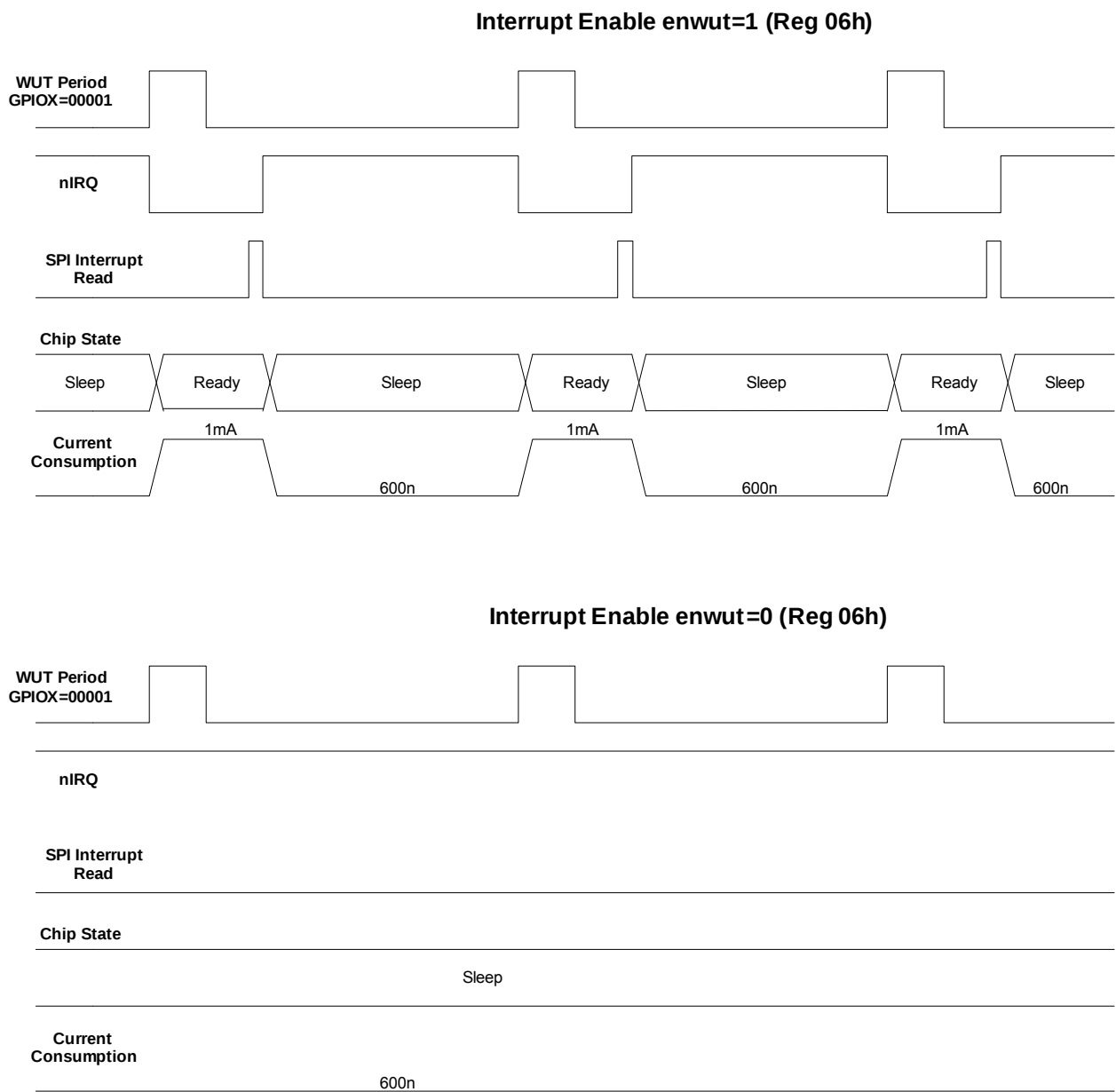
Figure 19. WUT Interrupt and WUT Operation
